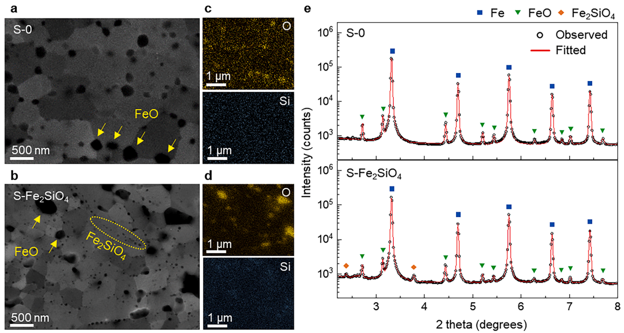
Fig. 5. Microstructure of as-fabricated composites. (a,b) SEM micrographs of (a) S-0 and (b) S-Fe 2 SiO 4 . A few FeO and Fe 2 SiO 4 particles are marked as an example. (c,d) EDS maps (oxygen and silicon) of (c) the region corresponding to (a) and (d) the region corresponding to (b). (e) High-energy XRD patterns of S-0 and S-Fe 2 SiO 4 . The X-ray wavelength used is 0.1173 Å.
