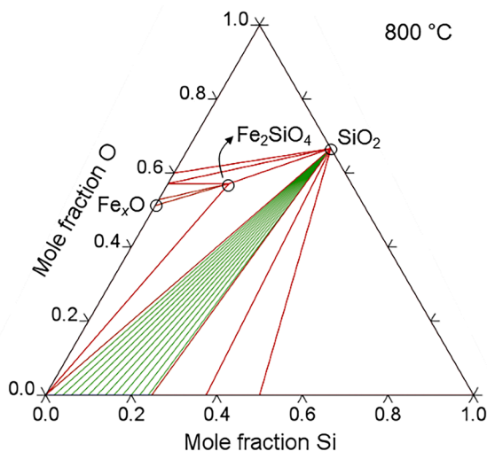
Fig. 4. Isothermal cross-section of Fe-Si-O ternary phase diagram at 800^\circ C .
