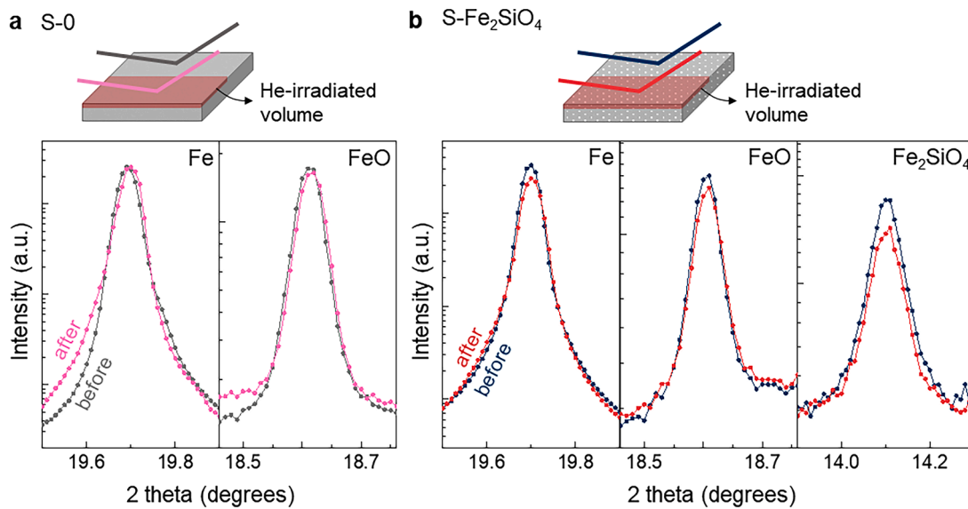
Fig. 6. Effect of helium irradiation on the crystal structure of the phases constituting the composites. (a,b) Grazing incidence XRD patterns of (a) S-0 and (b) S-Fe 2 SiO 4 comparing the position of the main XRD peaks of Fe, FeO, and Fe 2 SiO 4 before (gray and blue) and after (pink and red) helium irradiation.
