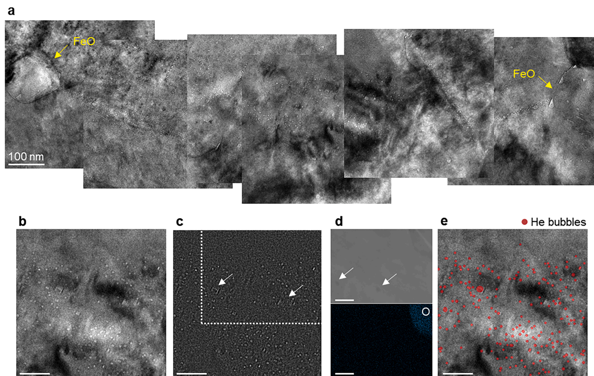
Fig. 8. Microstructural characterization of S-0 after irradiation with 5000 appm helium at 500 °C. (a) TEM micrographs of peak damage regions in S-0. (b) TEM micrograph showing the development of helium bubbles. (c) Preprocessed image of (b) to better visualize helium bubbles. (d) Enlarged STEM micrograph of the boxed region in (c) and corresponding STEM-EDS map. White arrows indicate the bubble-like features and the absence of oxygen signals from the STEM-EDS map. (e) TEM micrograph showing the detected helium bubbles, marked with red dots. Scale bars in (b–e), 50 nm.
