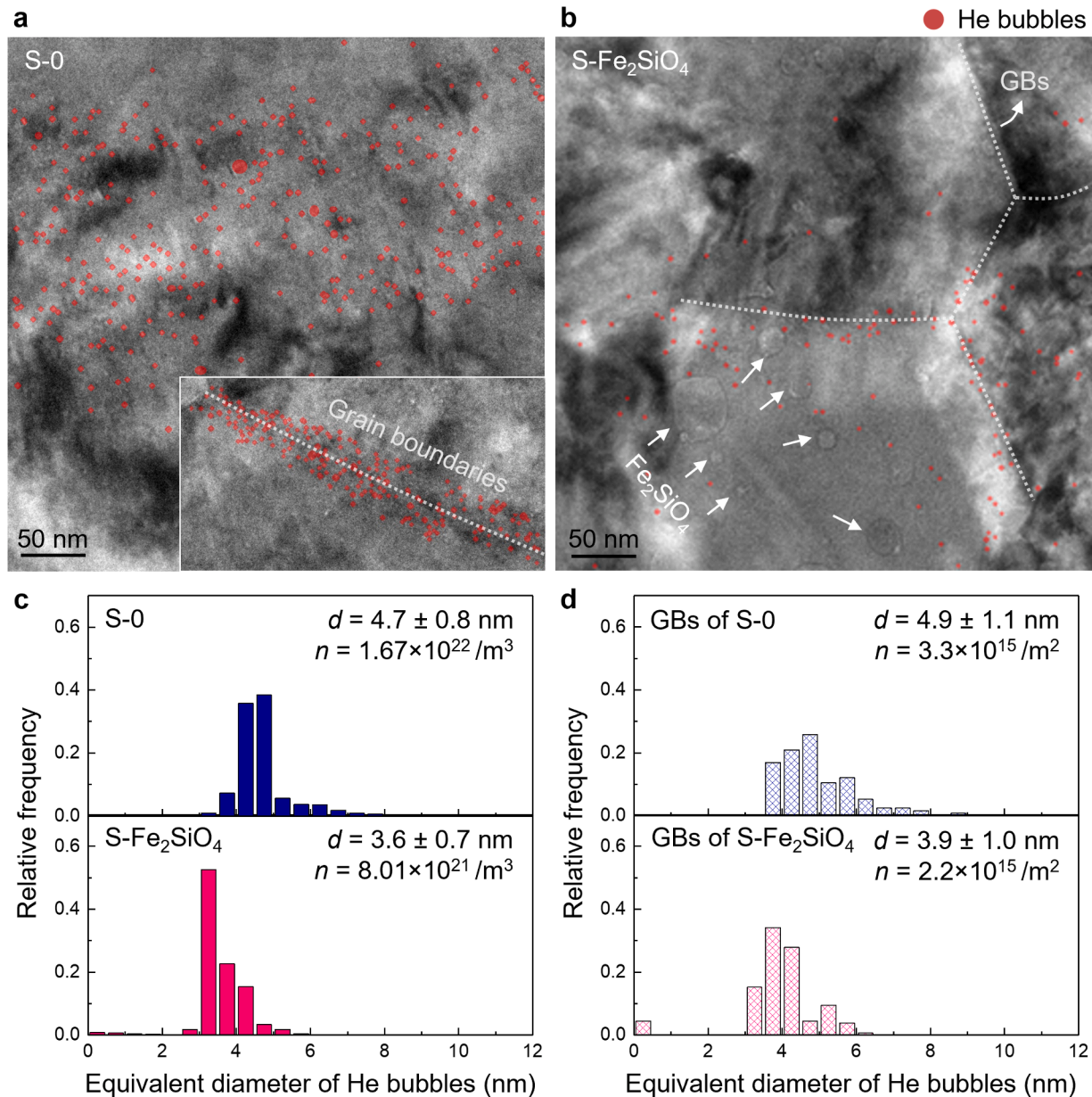
Fig. 10. Development of helium bubbles upon irradiation with 5000 apm helium at 500 °C. (a,b) TEM micrographs of a peak damage regions in (a) S-0 and (b) S-Fe 2 SiO 4 . Helium bubbles are highlighted in red and white dotted lines indicate grain boundaries. (c,d) Relative frequency of helium bubbles as a function of equivalent diameter in (c) the whole matrix of S-0 and S-Fe 2 SiO 4 and (d) the grain boundaries of S-0 and S-Fe 2 SiO 4 . d and n are the average diameter and the number density of helium bubbles, respectively.
