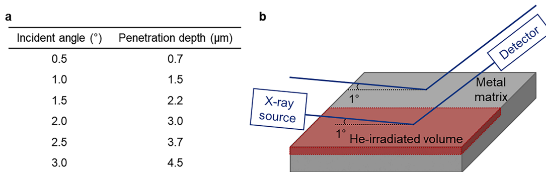
Fig. 2. Experimental conditions for grazing incidence X-ray diffraction. (a) Summary of incident angle and its corresponding penetration depth. The penetration depth was defined as the depth at which the relative intensity of X-ray ( I_s/I_0 , where I_s and I_0 are the intensities of the scattered and the incident X-rays, respectively) falls to 1 %. (b) Schematic diagram of the setup for grazing incidence X-ray diffraction experiments. The incident X-ray was directed at an angle of 1^\circ to achieve a \text{Fe}_2\text{SiO}_4 -to-helium ratio close to 1:1.
