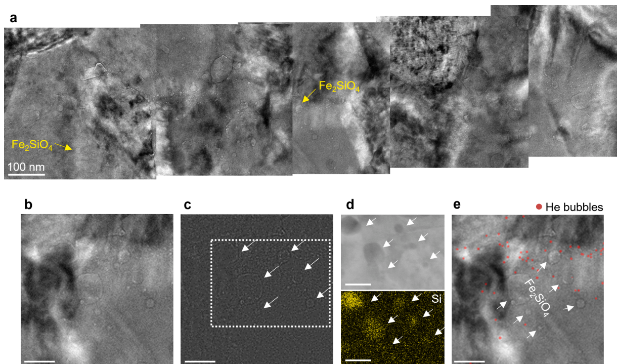
Fig. 9. Microstructural characterization of S- \text{Fe}_2\text{SiO}_4 after irradiation with 5000 appm helium at 500 \text{ }^\circ\text{C} . (a) TEM micrographs of peak damage regions in S- \text{Fe}_2\text{SiO}_4 . (b) TEM micrograph showing the development of helium bubbles. (c) Preprocessed image of (b) to better visualize helium bubbles. (d) Enlarged STEM micrograph of the boxed region in (c) and corresponding STEM-EDS map. White arrows indicate bubble-like features and the presence of silicon signals in the STEM-EDS map. (e) TEM micrograph showing the detected helium bubbles, marked with red dots. Scale bars in (b–e), 50 \text{ nm} .
