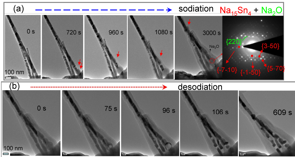
Figure S1 (a) TEM images showing the sodiation process and diffraction pattern at the region circled by red, showing the formation of \text{Na}_{15}\text{Sn}_4 and \text{Na}_2\text{O} after final sodiation; The diffraction pattern at the very right of the panel (a) shows the formation of \text{Na}_{15}\text{Sn}_4 core (red) and \text{Na}_2\text{O} (green) shell; and the red arrows label the location of the reaction fronts; (b) desodiation process at different times; The formation of \text{Na}_2\text{O} surface layer is the consequence of sodiation of \text{SnO}_2 and electron beam induced surface growth of Na species;
