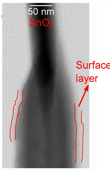
Figure S2 bright-field STEM image of the reaction front with the electron beam being blanked, showing much thinner \text{Na}_2\text{O} surface layer compared to Figure S1
