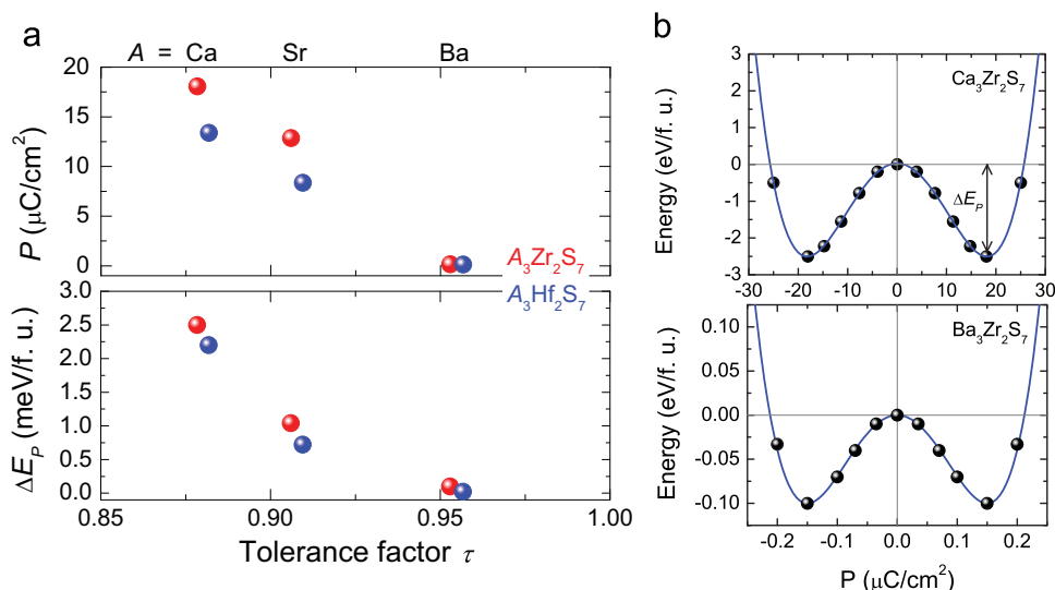
Fig. 3. (a) Spontaneous polarization ( P ) and ferroelectric stabilization energy (double-well potential depth, \Delta E_p ) for A_3B_2S_7 ( A=\text{Ca}, \text{Sr} and \text{Ba} , B=\text{Zr} and \text{Hf} ), sorted by the tolerance factor. (b) Simulated ferroelectric double well potential for \text{Ca}_3\text{Zr}_2\text{S}_7 and \text{Ba}_3\text{Zr}_2\text{S}_7 . Symbols are first-principles results and lines are fitted based on Landau model. \text{Ca}_3\text{Zr}_2\text{S}_7 has its P and \Delta E_p order of magnitude larger than those in \text{Ba}_3\text{Zr}_2\text{S}_7 .
