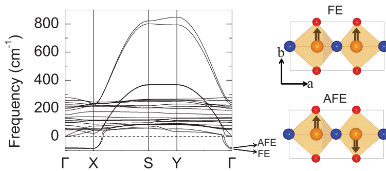
FigureS2: Calculated phonon spectrum for PE \text{NbOI}_2 monolayer. There are two unstable soft-phonon modes corresponding to ferroelectric (FE) and antiferroelectric (AFE) Nb polar displacement relative to the center of \text{NbO}_2\text{X}_4 octahedra along crystallographic b axis.
