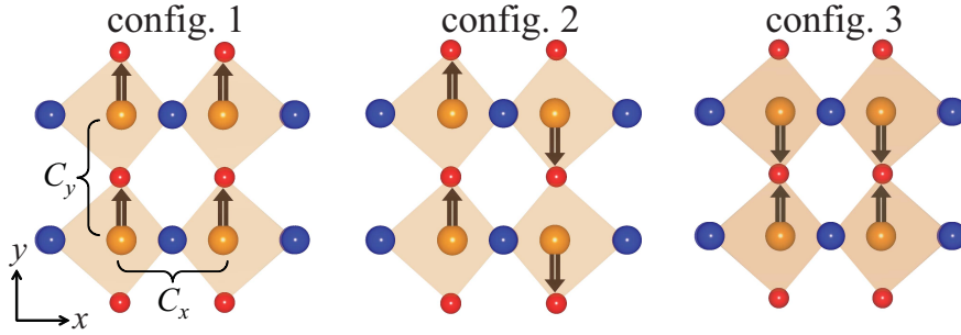
Figure S5: Three different polar configurations used to extract the polar displacement interaction parameters C_x and C_y appeared in Table 2 of the main text. Config. 1 and 2 correspond to FE and AFE phase for NbOX 2 monolayer, Config. 3 contains head-to-head (tail-to-tail) Nb polar arrangement, which is highly unfavorable. We constrain three configurations to have same Nb polar displacement amplitude ( |d_i|=d ). So that based on Eq. (2) of main text, their energy difference can be written as: E_2 - E_1 = 16C_x \cdot d^2 ; E_3 - E_1 = 16C_y \cdot d^2 . The obtained parameters C_y \gg C_x , owing to the very high energy cost to form head-to-head (tail-to-tail) polar arrangement.
