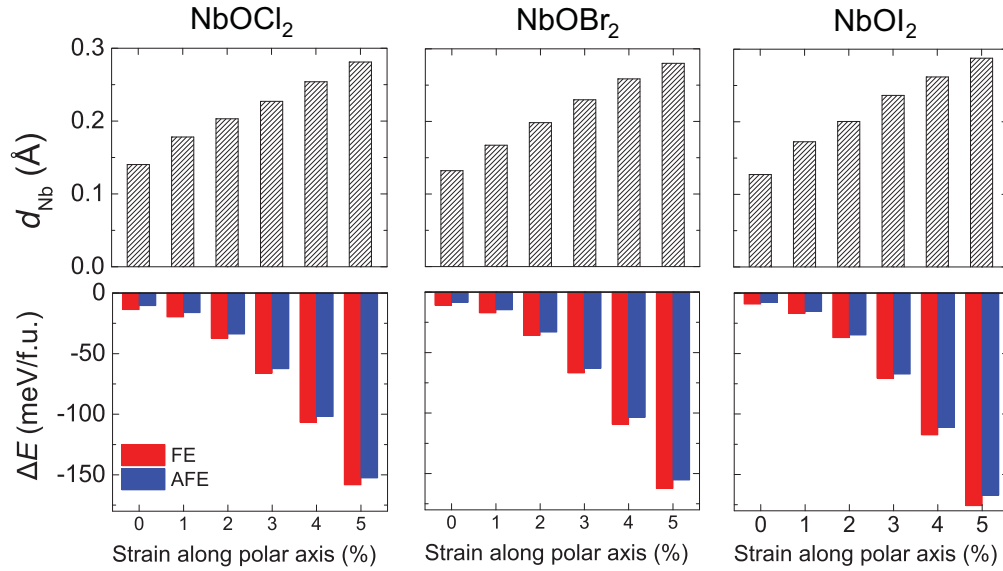
Figure S7: Variation of Nb polar displacement ( d_{\text{Nb}} ) in FE phase, the energy for FE and AFE phases relative to PE phase ( \Delta E ) of \text{NbOX}_2 monolayer as a function of tensile strain applied along the polar axis.
