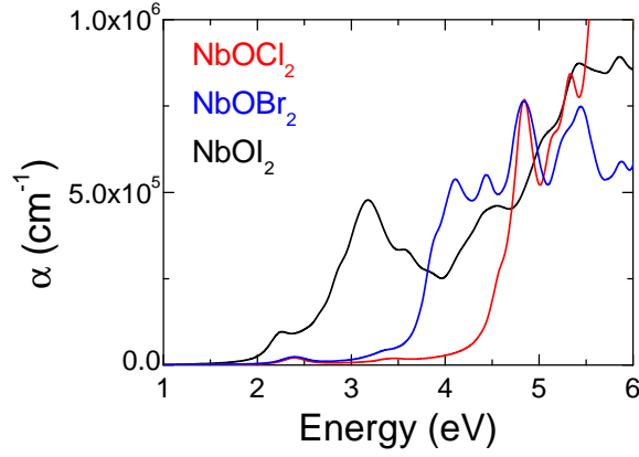
Figure S4: Optical absorption coefficient \alpha(\omega) for FE NbOX 2 bulk, calculated using HSE functional. Among the three bulk compounds, only NbOI 2 exhibits semiconducting optical absorption properties. As an indirect band gap semiconductor, NbOI 2 bulk can effectively absorb incident light with photon energy above 2.0 eV.
