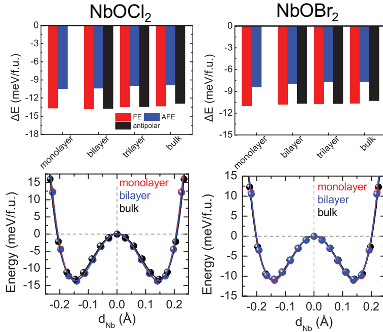
Figure S3: Upper panel: Variation of the total energy for different polar configurations in \text{NbOCl}_2 and \text{NbOBr}_2 systems as a function of layer numbers, where the energy of the corresponding PE phases are chosen as energy zero. The energy stability trends are: \text{FE} \approx \text{antipolar} > \text{AFE} . Lower panel: Nb polar displacement-energy double well plots connecting PE and two FE phases in \text{NbOCl}_2 and \text{NbOBr}_2 monolayer, bilayer and bulk. Symbols are the calculated results, lines are fitted to the data based on Landau model. Similar to \text{NbOI}_2 , both the magnitude of Nb polar displacement and spontaneous potential depth in FE \text{NbOCl}_2 and \text{NbOBr}_2 remain almost unchanged with respect to the layer numbers.
