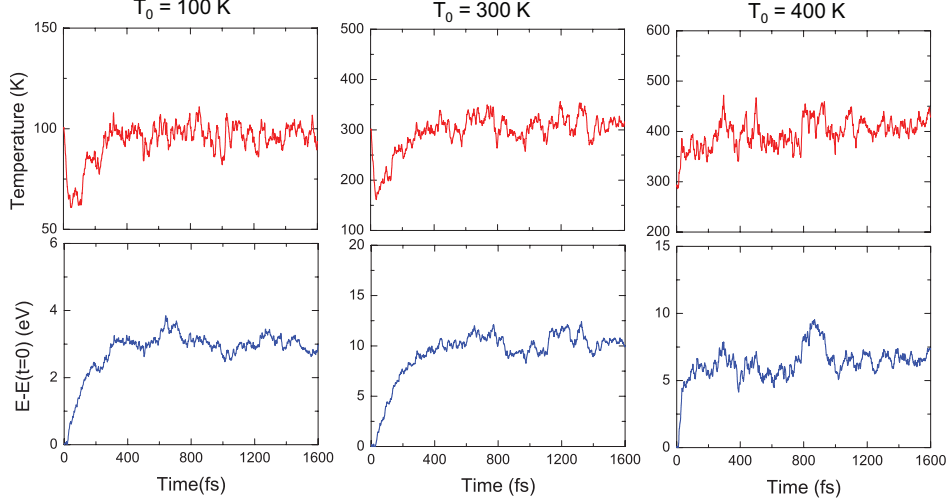
Figure S6: Full time evolution of the instantaneous temperature, total energies for NbOI 2 monolayer at the selected target temperature during ab initial MD simulations.
