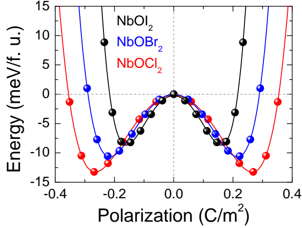
FigureS1: Energy-polarization double well profiles for FE bulk \text{NbOX}_2 . Energy evolution as a function of spontaneous polarization connecting the FE C2 and PE C2/m phases of \text{NbOX}_2 bulk. Symbols are the calculated results, and lines are fitted to the data based on Landau model. The trend in magnitude of spontaneous polarization and FE potential depth are \text{NbOI}_2 < \text{NbOBr}_2 < \text{NbOCl}_2 .
