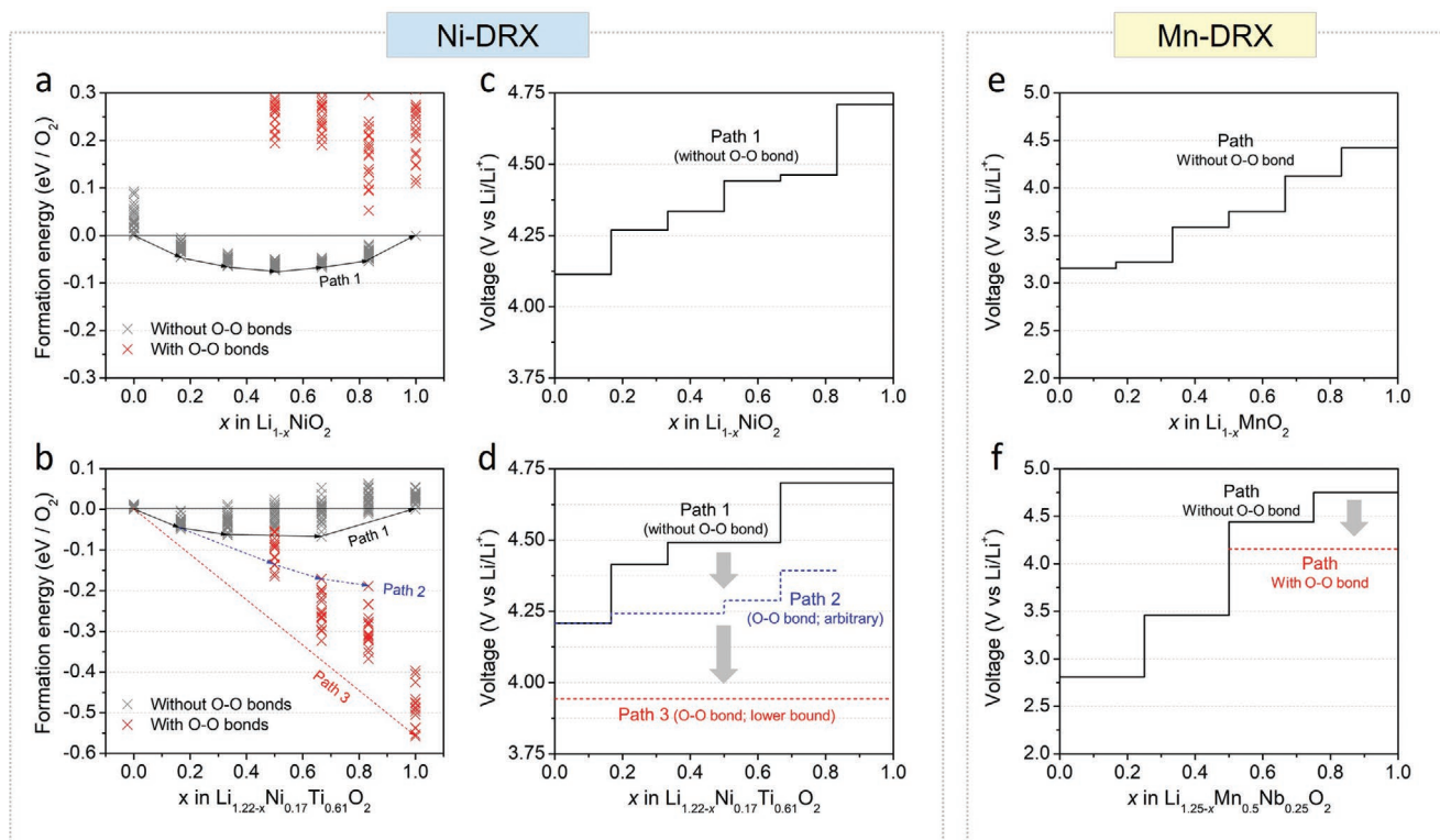
Figure 5. a,b) The DFT formation energies (eV/O 2 ) of various a) DRX Li 1-x NiO 2 and b) Li 1.22-x Ni 0.17 Ti 0.61 O 2 model structures as a function of the Li-extraction level ( x ). The gray and red points represent the energies of the structures without and with the short O–O bonds (formed upon AIMD simulation at 1500 K), respectively. Path 1 in the Figure corresponds to Li-extraction, which would not lead to the O–O bond formation. Paths 2 (arbitrary) and Path 3 (the lowest voltage path) in Figure 5b involve O–O bond formation upon O-oxidation. c,d) The DFT voltage profiles of c) DRX LiNiO 2 and d) Li 1.22-x Ni 0.17 Ti 0.61 O 2 constructed based on different paths. e,f) The DFT voltage profile of e) DRX LiMnO 2 and f) Li 1.25-x Mn 0.5 Nb 0.25 O 2 . For Li 1.25-x Mn 0.5 Nb 0.25 O 2 , voltage profiles taking two different paths were shown as the O–O bond formation can decrease its voltage while it is not for DRX LiMnO 2 .
