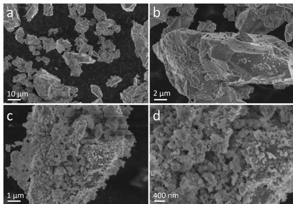
Figure S2. Scanning electron microscopy images of the (a, b) as-made and (c, d) ball-milled M90. The as-made M90 form into 5\ \mu\text{m} < d < 20\ \mu\text{m} particles; yet, ball milling pulverizes the particles into d < 200\ \text{nm} nanoparticles that loosely segregate into slightly larger particles with varying sizes. This particle size reduction upon ball mill is consistent with the XRD peak broadening after the ball milling.
