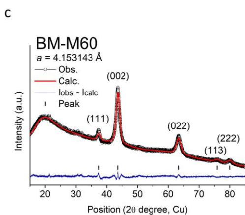
Figure S3. The XRD refinement and structural parameters of the (a, b) as-made and (c, d) ball-milled \text{Li}_{1.20}\text{Mn}_{0.60}\text{Nb}_{0.20}\text{O}_2 (M60). The same refinement protocol as described in the caption of Figure S1 was used.
