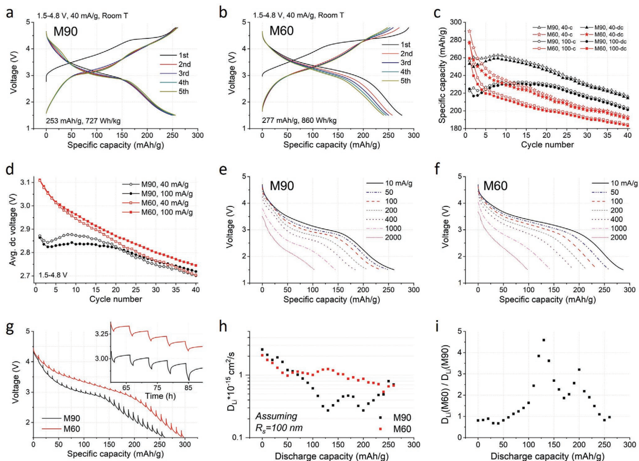
Figure 2. The initial five-cycle voltage profiles of a) M90 and b) M60 when they are cycled at 40 \text{ mA g}^{-1} between 1.5 and 4.8 V. c) The capacity retention of M90 and M60 during the 40 and 100 \text{ mA g}^{-1} cycling tests. d) The average discharge voltage of M90 and M60 upon cycling ( 40 or 100 \text{ mA g}^{-1} , 1.5–4.8 V). The discharge profiles of e) M90 and f) M60, when they are charged at 20 \text{ mA g}^{-1} and then discharged at different rates (10, 50, 100, 200, 400, 1000, and 2000 \text{ mA g}^{-1} ). g) The discharge portion of the galvanostatic intermittent titration technique (GITT) profiles of M90 and M60, shown as a function of discharge capacity. The inset zooms in the portion of the M90's GITT profile shown as a function of time (hours). h) The calculated Li-diffusivities of M90 and M60 based on the GITT results and i) their ratio.
