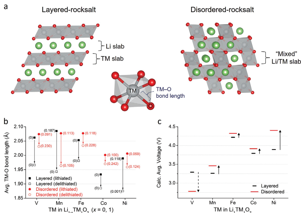
Figure 4. a) The schematics of the layered- and disordered-rocksalt (DRX) structures and TM–O octahedron. b) The computed average TM–O bond length in the layered- or DRX-Li 1-x TM 1 O 2 (TM = V, Mn, Fe, Co, Ni) before ( x = 0 ) and after delithiation ( x = 1 ): The standard deviations are shown in parentheses. c) The computed average voltage of the layered- or DRX-Li 1-x TM 1 O 2 (TM = V, Mn, Fe, Co, Ni).
