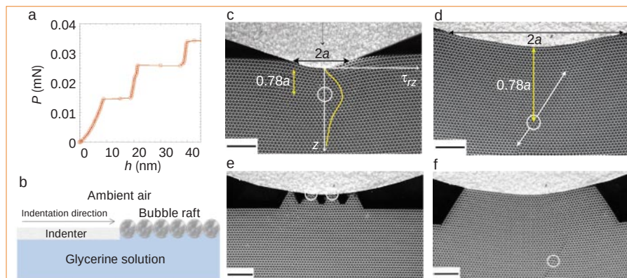
Figure 1 Dislocation nucleation during nanoindentation. a , Indentation load, P , plotted against depth, h , in (133) single-crystal aluminium, showing elastic deformation separated by displacement bursts attributed to dislocation nucleation 3 . b , Diagram of bubble-raft indentation. c , d , Initially defect-free rafts in which dislocation nucleation is induced by loading with indenters of different tip radii but at the same normalized depth, z = 0.78 a (white circle), where a is half the width of the contact. This is the position of maximum shear stress, \tau_{rz} , shown in c . Nucleation (white circle) of a dislocation dipole is seen in d : one dislocation proceeds to the surface and the other into the crystal (white arrows). e , Indentation of atomic-scale asperities, showing plasticity (white circles) at the surface. f , Indentation of surface ledges of width comparable to the indenter radius causes dislocation nucleation within the crystal (white circle). Scale bar, 10 mm (representing 3 nm in our analogy).
