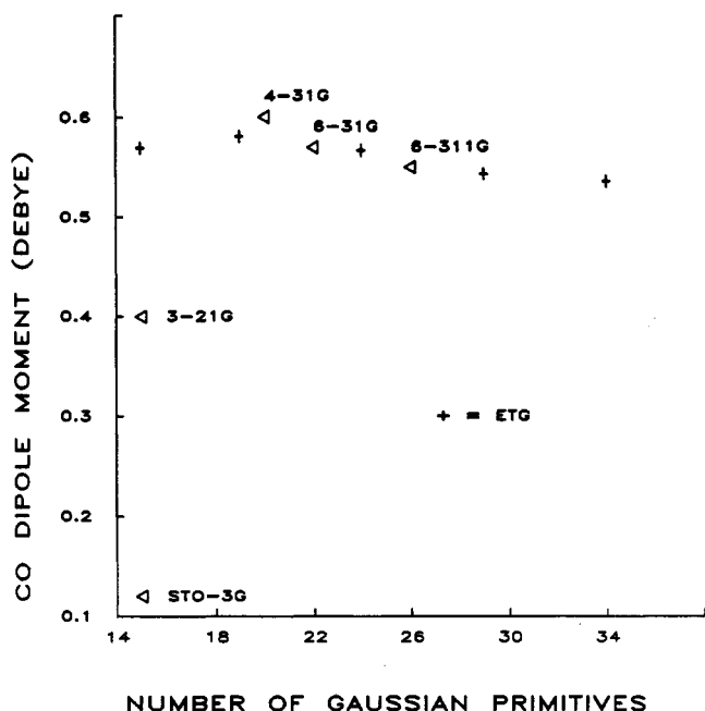
Figure 2. Variation in the SCF dipole moment of carbon monoxide as a function of the number of gaussian primitives for various basis sets.
