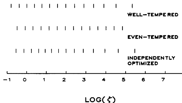
Figure 1. The distribution of s-symmetry gaussian exponents in three energy-optimized (14s,9p) neon atom basis sets.
