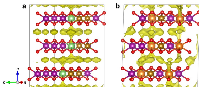
Fig S15. The BV calculations for de-sodiated (a) O3- \text{Na}_{0.83}\text{Li}_{0.17}\text{Fe}_{0.33}\text{Mn}_{0.5}\text{O}_2 (NaLFM) and (b) \text{Na}_{0.83}\text{Mg}_{0.33}\text{Fe}_{0.17}\text{Mn}_{0.5}\text{O}_2 (NaMFM) systems. For NaMFM system, the calculations were based on the supercell obtained by 2 \times 3 \times 1 expansion of the conventional cell O3- \text{NaFeO}_2 (R-3m), including 15 Na, 6 Mg, 3 Fe, 9 Mn and 36 O atoms.
