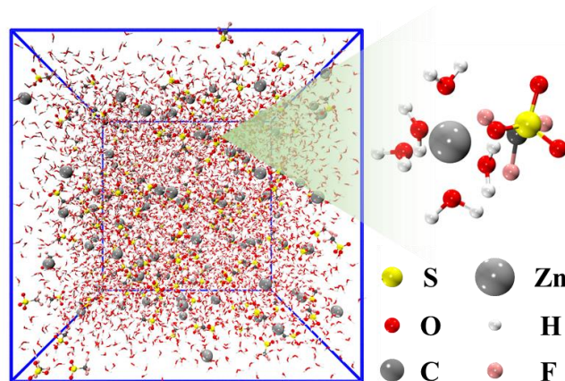
Figure S5. 3D snapshot obtained by MD simulations and representative \text{Zn}^{2+} -solvation structure of DES0.
