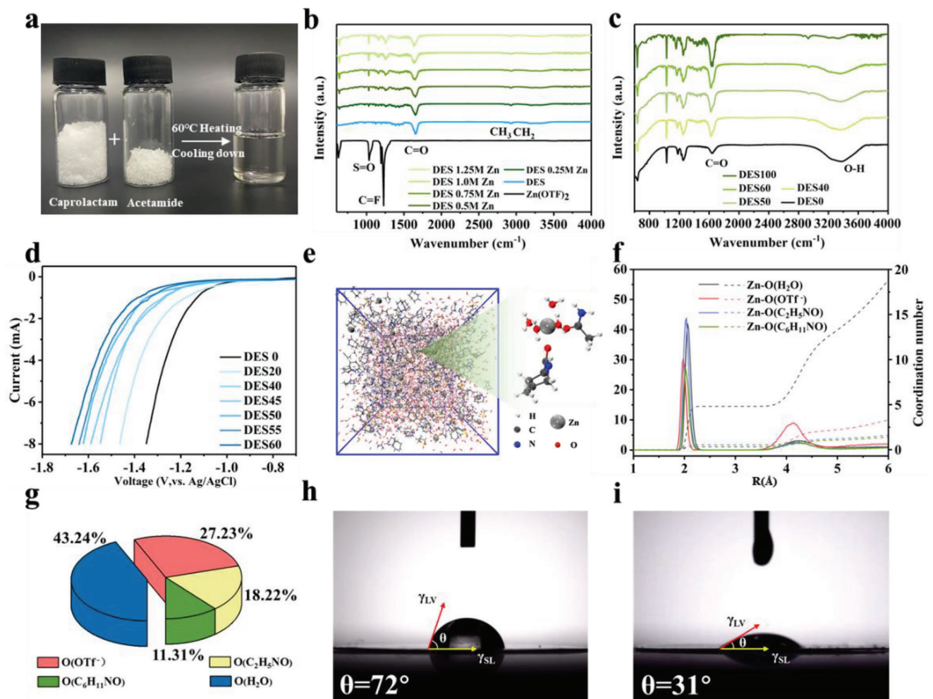
Figure 1. Eutectic electrolyte structure analysis a) Formation process of deep eutectic solvent; FT-IR spectra of DES b) with gradient concentration of \text{Zn}(\text{OTf})_2 ; c) with 1 M \text{Zn}(\text{OTf})_2 adding gradient volume fraction of \text{H}_2\text{O} ; d) LSV curve of Zn anode in different DES electrolytes at a scan rate of 1 \text{ mV s}^{-1} ; e) 3D snapshot obtained by MD simulations and representative \text{Zn}^{2+} -solvation structure of DES50; f) RDFs for \text{Zn}-\text{O}(\text{H}_2\text{O}) , \text{Zn}-\text{O}(\text{OTf}^-) , \text{Zn}-\text{O}(\text{C}_2\text{H}_5\text{NO}) , \text{Zn}-\text{O}(\text{C}_6\text{H}_{11}\text{NO}) with a coordination number of \text{Zn}^{2+} from MD simulations and g) distribution of coordination in primary solvation sheath in DES50. The contact angle of h) DES0 and i) DES50 in Zn foils.
