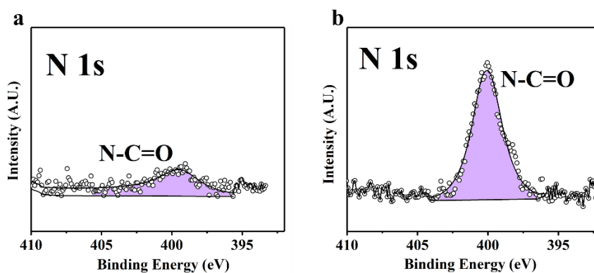
Figure S19. XPS spectra of N 1s of Zn foils surface soaking in a) DES0 and b) DES50 electrolytes for 14 days.
