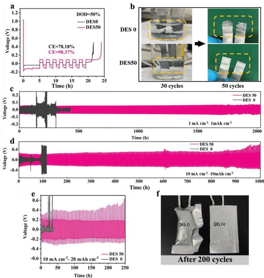
Figure 4. a) The comparison of Coulombic efficiency in DES0 and DES50 electrolytes at 50% DOD; b) Digital photograph of Zn foils cycling in DES0 and DES50 electrolyte for 30 cycles and 50 cycles at a current of 1 \text{ mA cm}^{-2} and a capacity of 1 \text{ mAh cm}^{-2} ; Long-term galvanostatic cycling of Zn||Zn symmetric cell with DES50 and DES0 electrolytes at c) 1 \text{ mA cm}^{-2} - 1 \text{ mAh cm}^{-2} ; d) 10 \text{ mA cm}^{-2} - 10 \text{ mAh cm}^{-2} and e) 10 \text{ mA cm}^{-2} - 20 \text{ mAh cm}^{-2} ; f) Macroscopic flatulence of pouch cells in DES0 and DES50 electrolyte.
