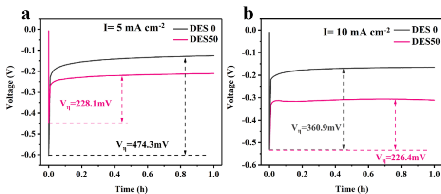
Figure S21. Nucleation overpotential of Zn anode in DES50 and DES0 at a current of a) 5 \text{mA cm}^{-2} and b) 10 \text{mA cm}^{-2} .
