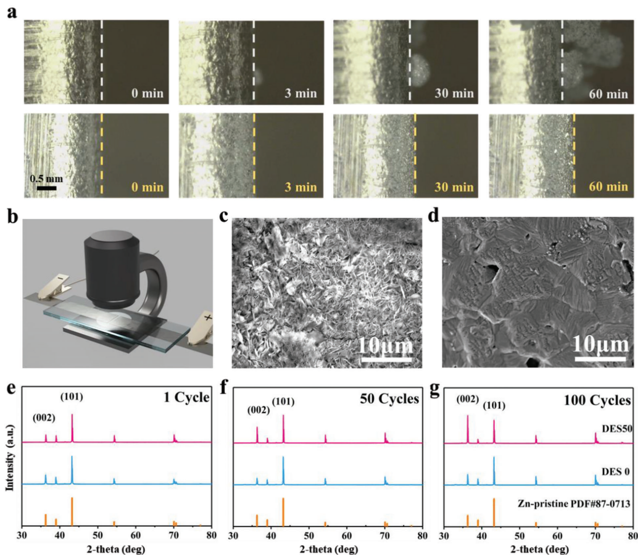
Figure 3. Zn plating/stripping and deposition behaviors. a) In situ optical microscopic observation of dendrite growth in DES0 and DES50 at a current of 20 \text{ mA cm}^{-1} ; b) schematic diagram of in situ microscopic observation equipment. Comparison of SEM images of Zn anode surface after 100 cycles in c) DES0 and d) DES50 at 1 \text{ mA cm}^{-2} with a capacity of 1 \text{ mAh cm}^{-2} and XRD patterns of Zn anode after e) 1 cycle; f) 50 cycles and g) 100 cycles.
