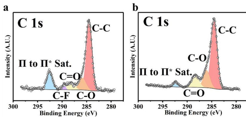
Figure S20. XPS spectra of C 1s of Zn foils surface soaking in a) DES0 and b) DES50 electrolytes for 14 days.
