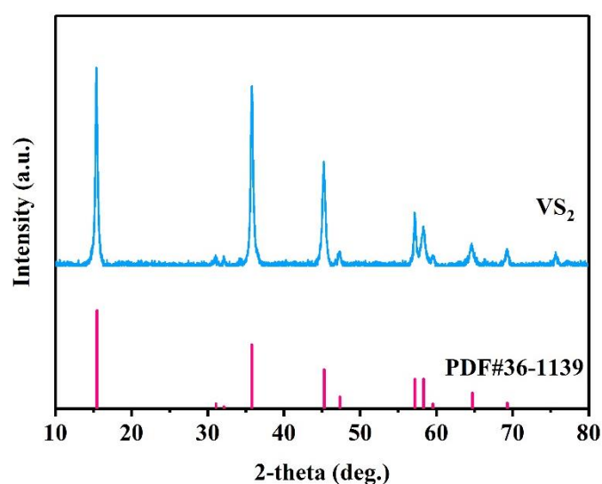
Figure S27. XRD pattern of VS 2 cathode materials.
