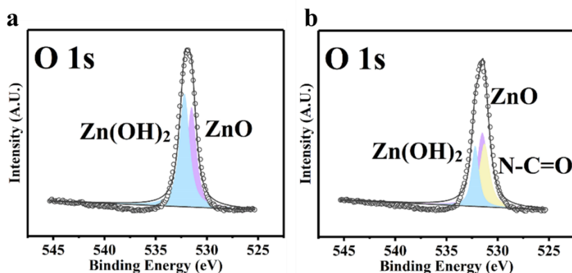
Figure S18. XPS spectra of O 1s of Zn foils surface soaking in a) DES0 and b) DES50 electrolytes for 14 days.
