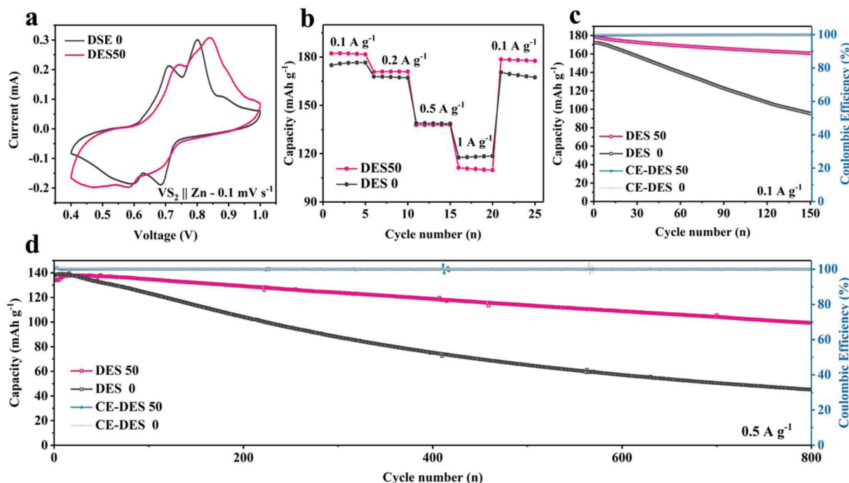
Figure 5. Electrochemical performance of \text{VS}_2||\text{Zn} cells operated in DES50 and DES0. a) CV curves of \text{VS}_2 cathode; b) Rate performance; c,d) Long-term cycling performance of \text{VS}_2||\text{Zn} full cell at 0.1 \text{ A g}^{-1} and 0.5 \text{ A g}^{-1} .
