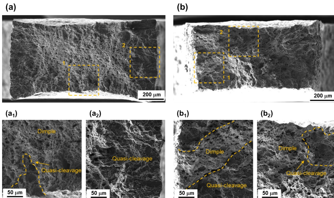
Fig. S3 Fractography of the tensile tested samples. (a) ECD treated for 30 minutes. (b) ECD treated for five hours. The figures below are the magnified images of the area marked in dotted boxes.
