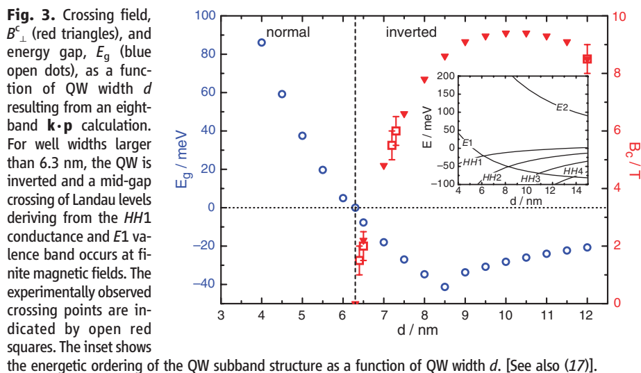
Fig. 3. Crossing field, B_c^\perp (red triangles), and energy gap, E_g (blue open dots), as a function of QW width d resulting from an eight-band \mathbf{k}\cdot\mathbf{p} calculation. For well widths larger than 6.3 nm, the QW is inverted and a mid-gap crossing of Landau levels deriving from the HH1 conduction and E1 valence band occurs at finite magnetic fields. The experimentally observed crossing points are indicated by open red squares. The inset shows the energetic ordering of the QW subband structure as a function of QW width d . [See also (17)].
