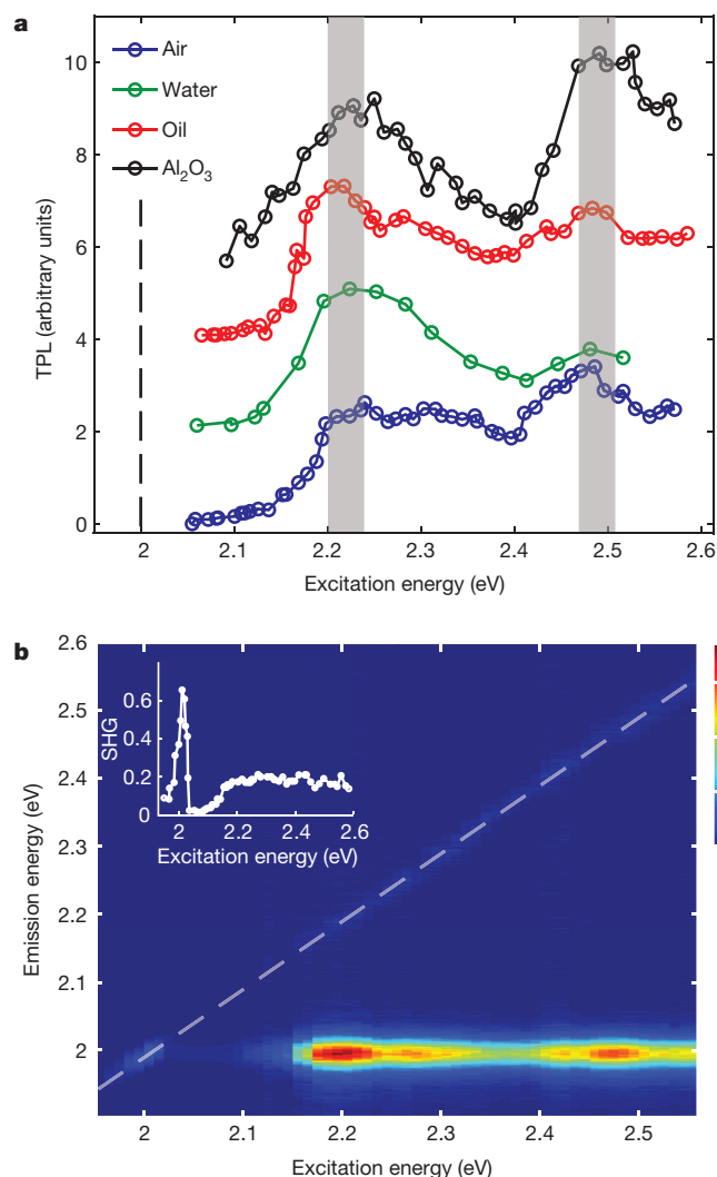
Figure 4 | Excitonic energy levels are robust to changes in the dielectric environment and to temperature changes. a , Room-temperature two-photon spectra of single-layer \text{WS}_2 with different top capping layers that tune the dielectric environment immediately adjacent to the atomic layer. The curves respectively represent the uncapped ( \epsilon_{\text{ave}} = 1.625 , where \epsilon_{\text{ave}} is the average dielectric constant between capping layers and the substrate), water capped ( \epsilon_{\text{ave}} = 1.97 ), immersion-oil capped ( \epsilon_{\text{ave}} = 2.25 ) and \text{Al}_2\text{O}_3 capped ( \epsilon_{\text{ave}} = 2.57 ) samples, and each curve is adjusted to a similar vertical scale and shifted for better visualization. The emission peak is at 2 eV, marked by the vertical black dashed line. Evidently, the 2p and 3p peak positions remain roughly unchanged within experimental error, marked by the grey bands at 2.22 \pm 0.02 eV and 2.49 \pm 0.02 eV, respectively. Therefore, the 1s – np ( n = 2, 3 ) separation is approximately the same as the low-temperature uncapped result (Fig. 2), suggesting that the excitation energy of the low-energy exciton levels are relatively insensitive to dielectric environmental and temperature perturbations, as discussed in the main text. b , Main panel: measured emission spectra at different excitation energies of an immersion-oil capped \text{WS}_2 monolayer at room temperature. The horizontal line signal is the TPL emission, with two hotspots along the line corresponding to the 2p and 3p two-photon absorption peaks. Colour scale represents the normalized emission intensity. The SHG signal due to the broken inversion symmetry in the monolayer is observed (along the dashed line as an eye guide). At the intersection between the SHG and TPL line, the SHG signal experiences an excitonic enhancement from the A exciton 1s state (inset).
